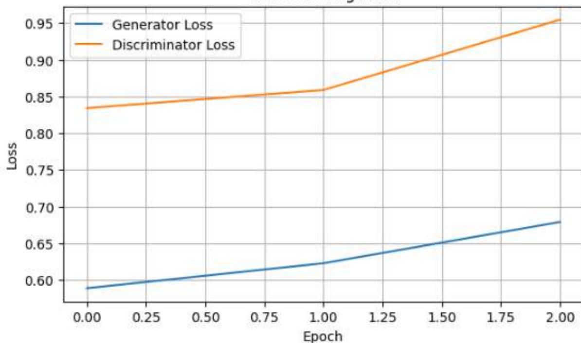
GAN Training Loss
